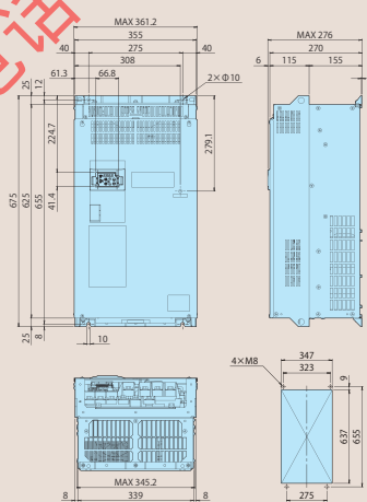
FRN0168E2S-4C
