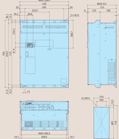
FRN0240E2S-4C, FRN0290E2S-4C
